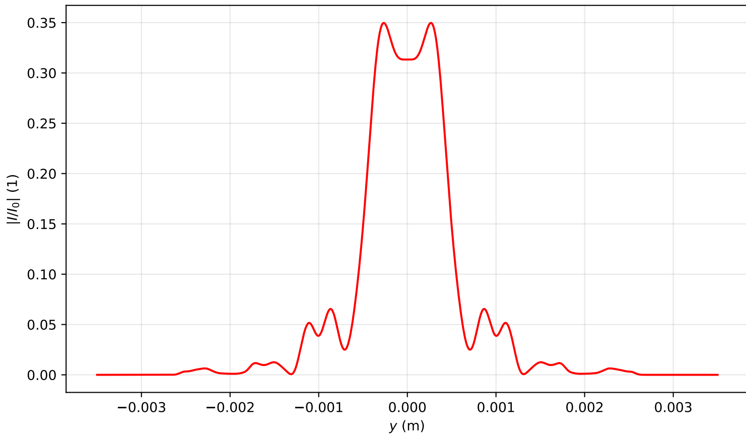
Intensity profile I(x=0, y, z=1.911)/I_0 , P_{in}=5.5P_{cr} , artificial time
